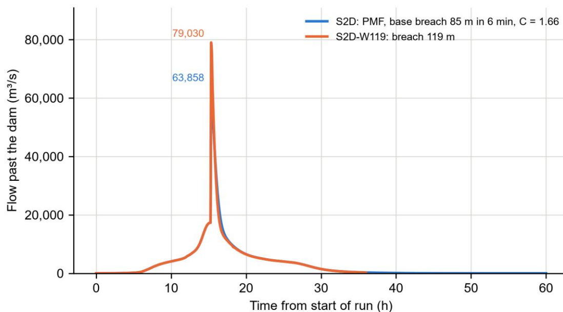
Figure 25 - Flow past the dam for the flood-day breach-width runs.
