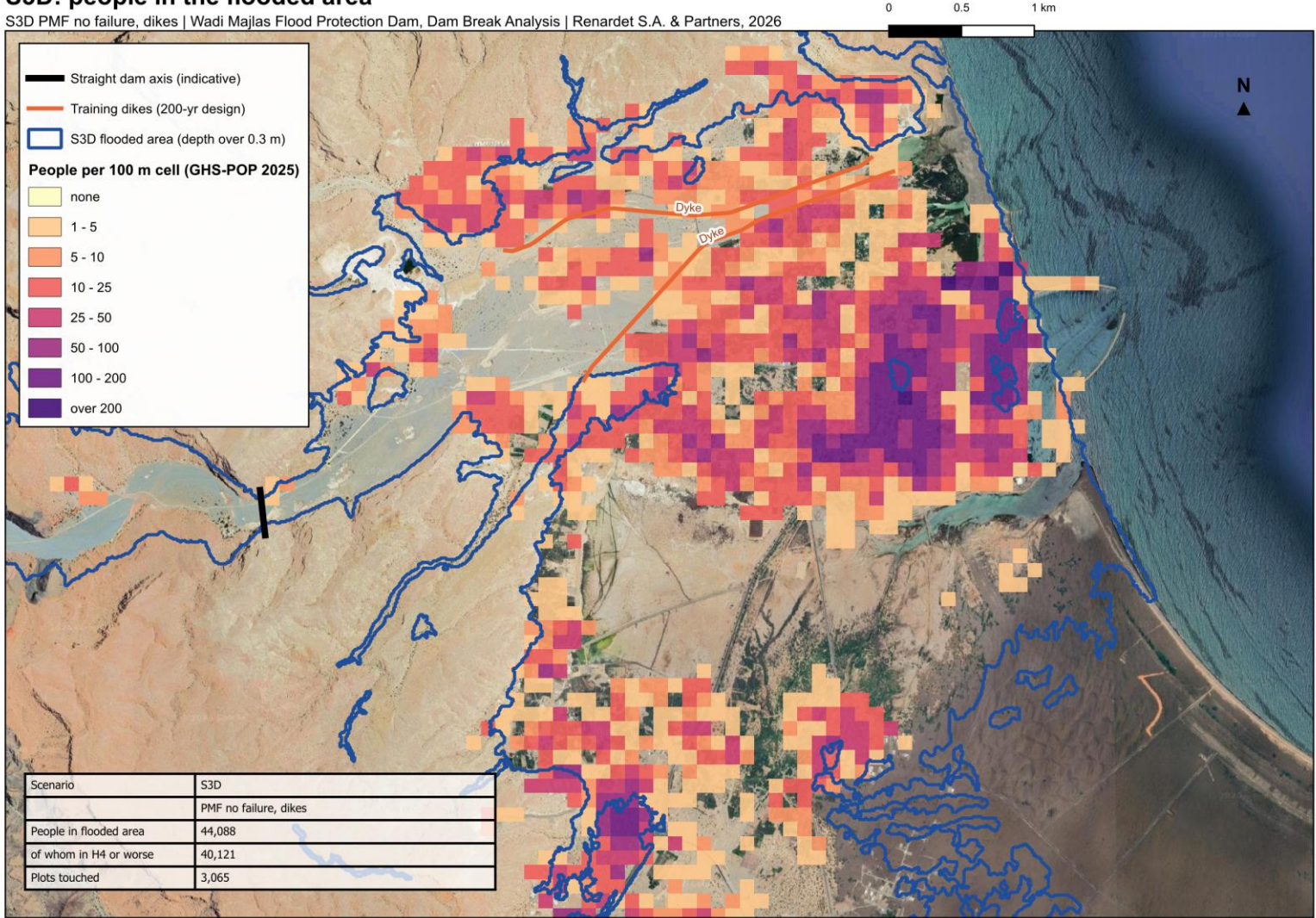
Figure 31 - S3D: people per 100 m cell (GHS-POP 2025) with the flooded area outlined.
