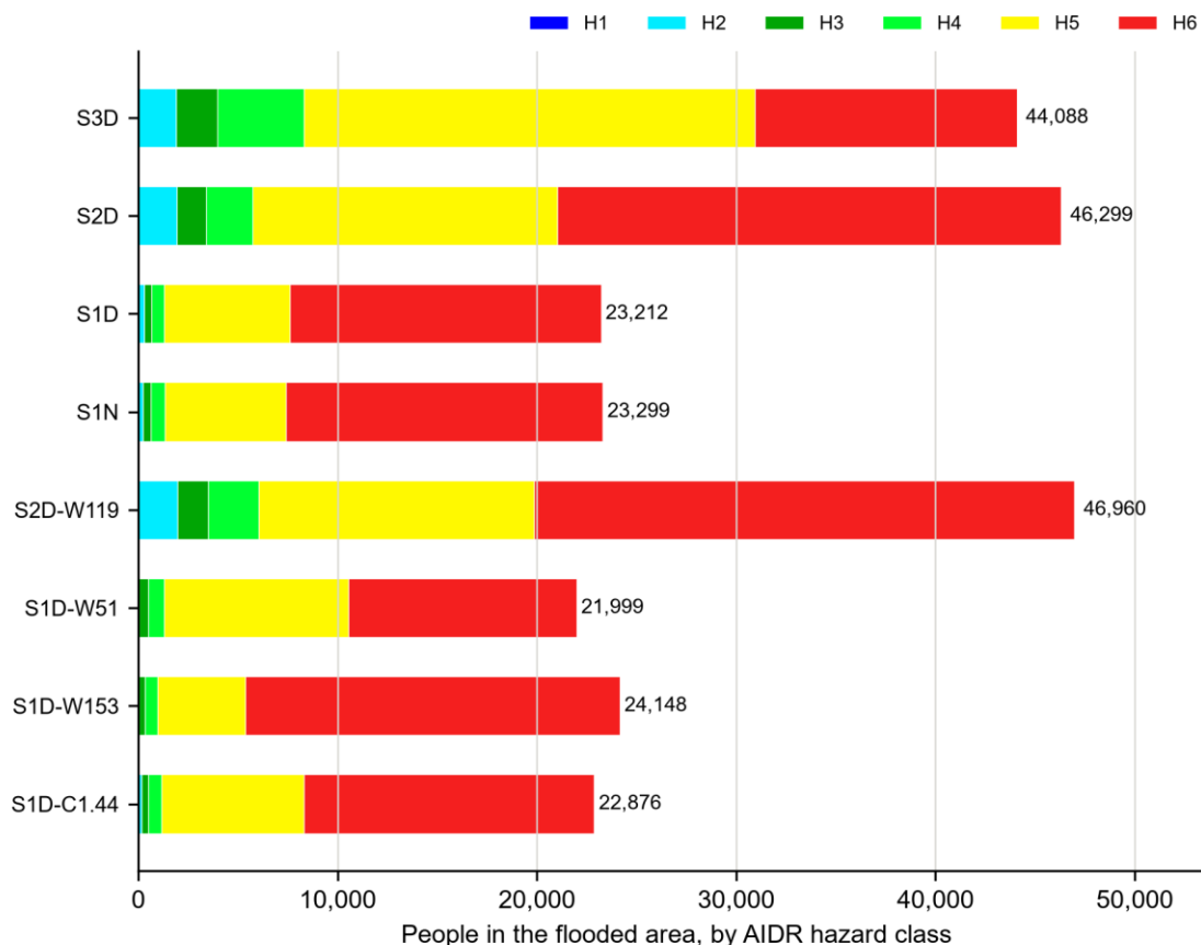
Figure 27 - People in the flooded area by hazard class, per scenario.
