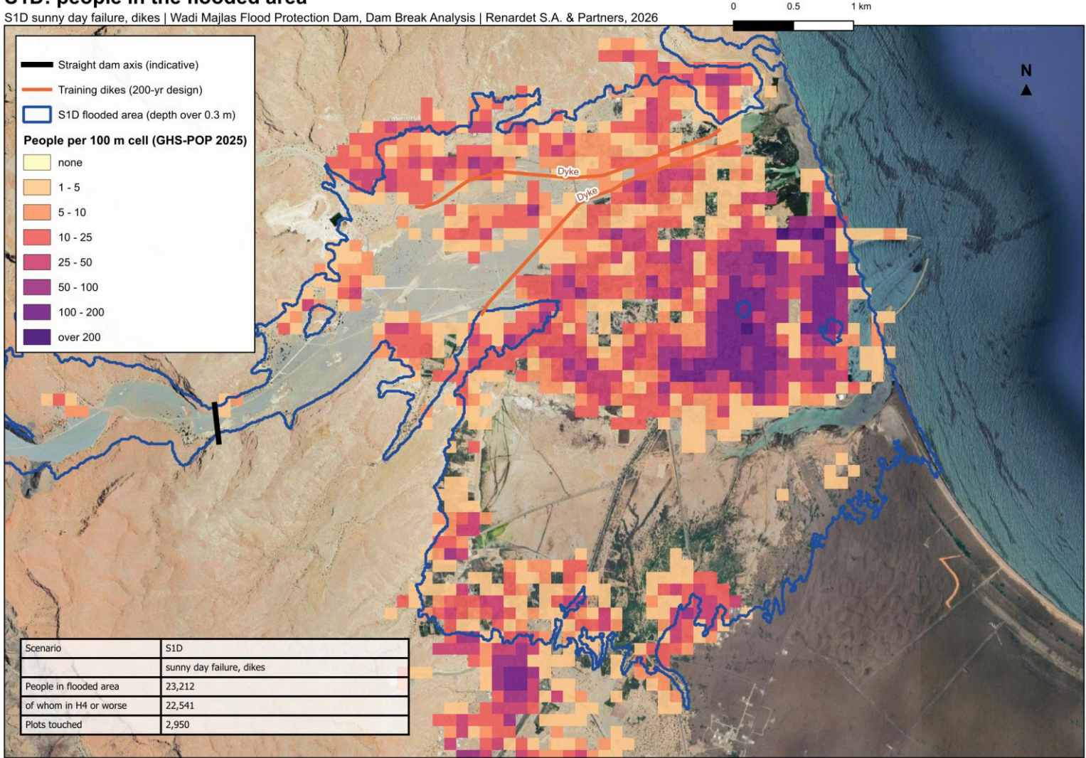
Figure 29 - S1D: people per 100 m cell (GHS-POP 2025) with the flooded area outlined.
