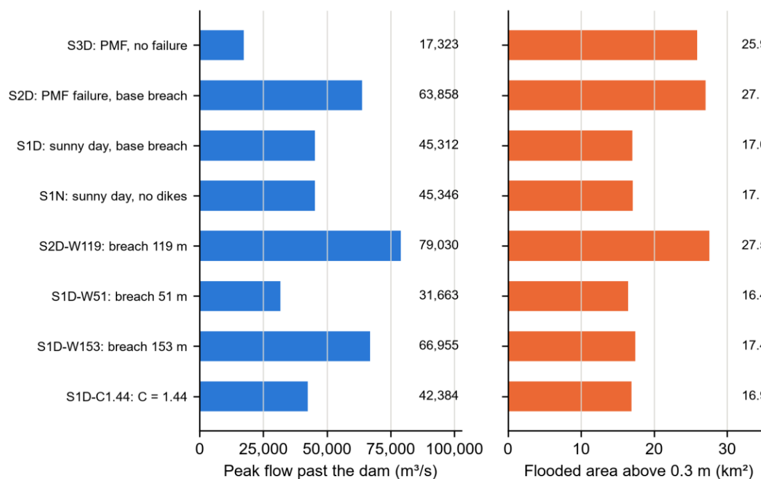
Figure 26 - Peak flow and flooded area of all runs.
