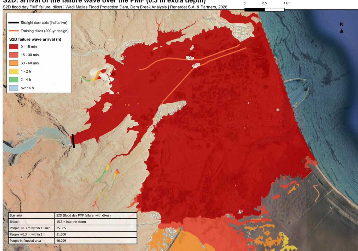
Figure 32 - S2D: arrival of the failure wave over the PMF, the time after the breach at which the water is 0.3 m deeper than without failure.
